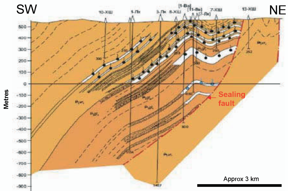
Cross-Section Line II-II (see Figure 5)
