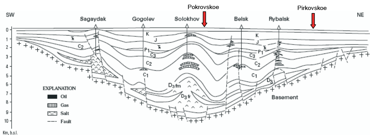
Dniepr-Donets Basin Location Map and Cross-Section
